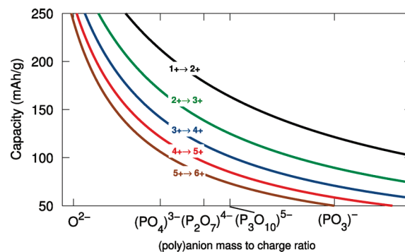
Figure 2. Best achievable gravimetric capacity for different \text{M}^{(n-1)+}/\text{M}^{n+} couples as a function of the mass-to-charge ratio of the (poly)anion. Oxides and different phosphate polyanions are indicated on the mass-to-charge ratio axis. For the sake of comparison, this plot assumes the mass of iron for the M element.
